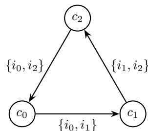
(b) Deviation graph G_\alpha(I) , \alpha < 2
